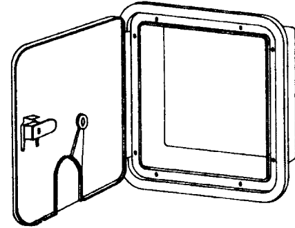
50 AMP POWER CORD HATCH CUTOUT: 6-3/8W X 6-7/8H OUTSIDE: 8W X 8-1/2H
