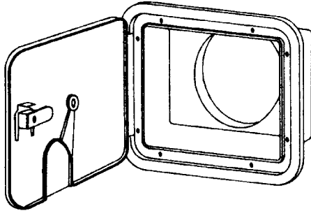
POWER CORD HATCH ROUGH OPENING: 6" W X 4-3/4" H OUTER FRAME: 7-1/2" X 6-1/2" H
