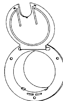
ROUND HATCH W/O BACK CUTOUT: 3-1/2 DIA. OUTSIDE: 4-1/2 DIA.
